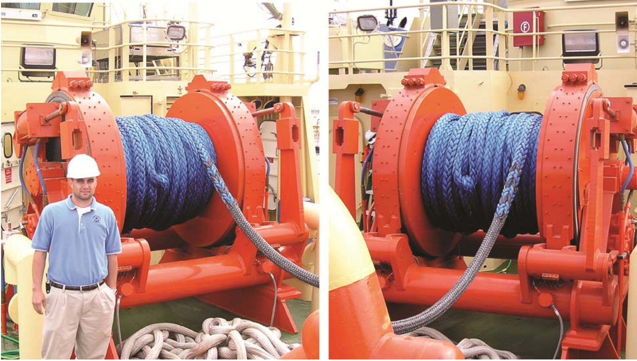
Markey Model DYS-52 (8x units), Edison Chouest Offshore, Cheniere/Freeport LNG (Cheniere Energy)
