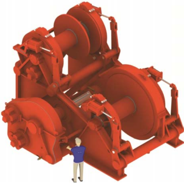
Markey Model DESDF-48WF-760HP (4x units), SMBC, Energia Costa Azul LNG, (Sempra Energy)
